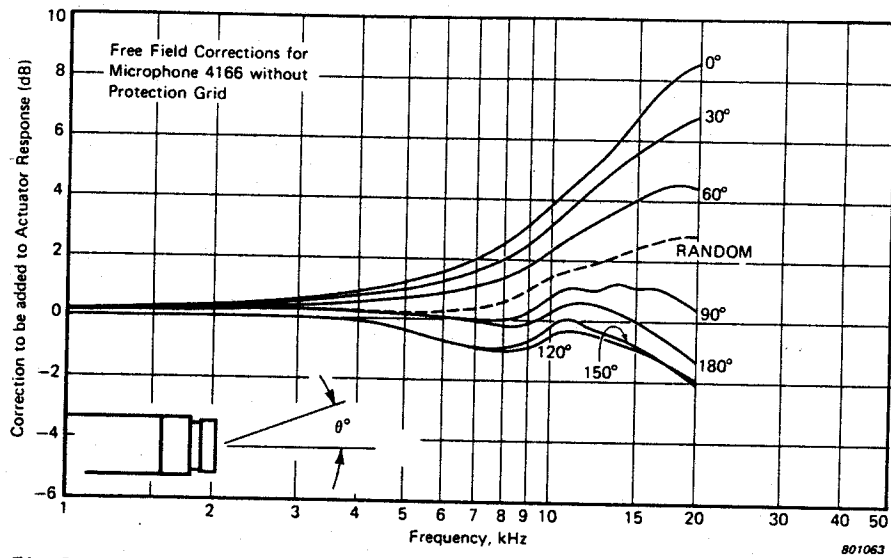
Fig.6.7. Free-field correction curves for half-inch Condenser Microphone Type 4166 without normal protection grid
